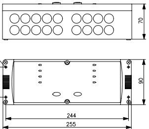
HTFRD-316.125 / HTFRL-316.125
